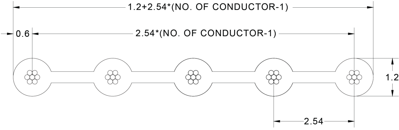
TYPE A
