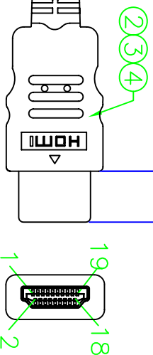
Conn.2 HDMI A Type Male Molding
