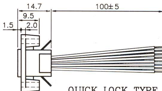
QUICK LOCK TYPE (MDC-173~MDC-178)
