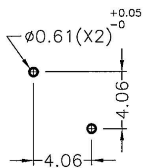
MOUNTING HOLE
