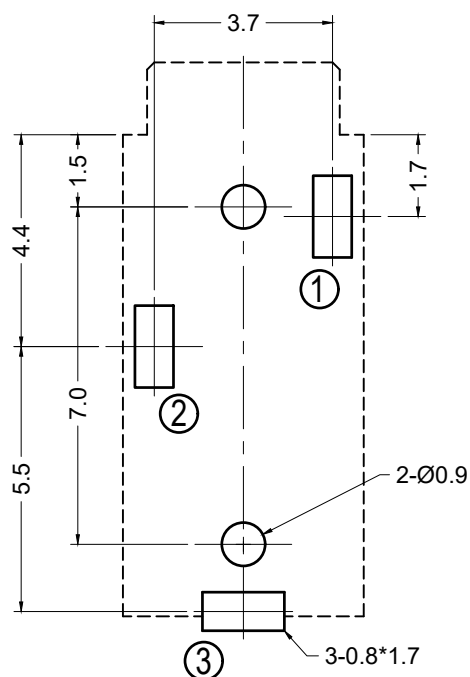
Recommended PCB Layout (Bottom View)
