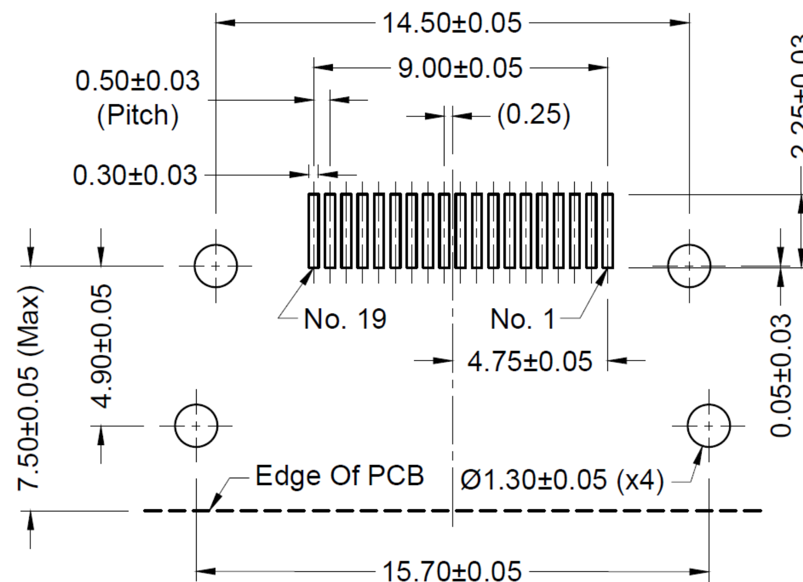
Recommended PCB Layout
