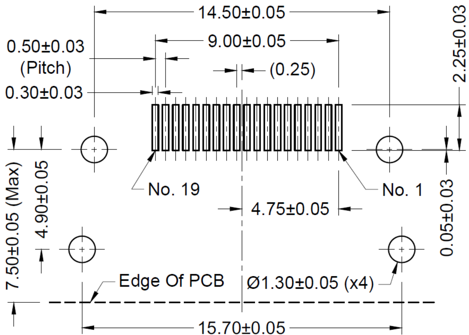
Recommended PCB Layout
