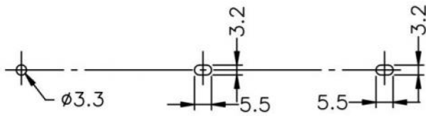
MOUNTING HOLES
