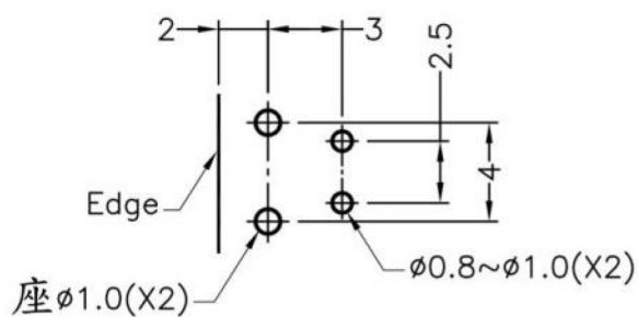
MOUNTING HOLE
