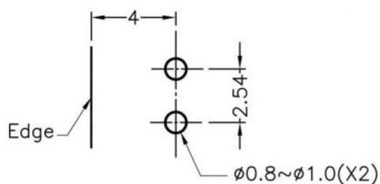
MOUNTING HOLES
