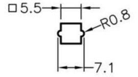
MOUNTING HOLE
